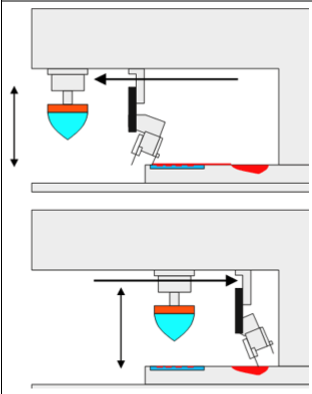
OPEN INK TROUGH WITH INKING MECHANISM MOUNTED ABOVE THE PLATE
