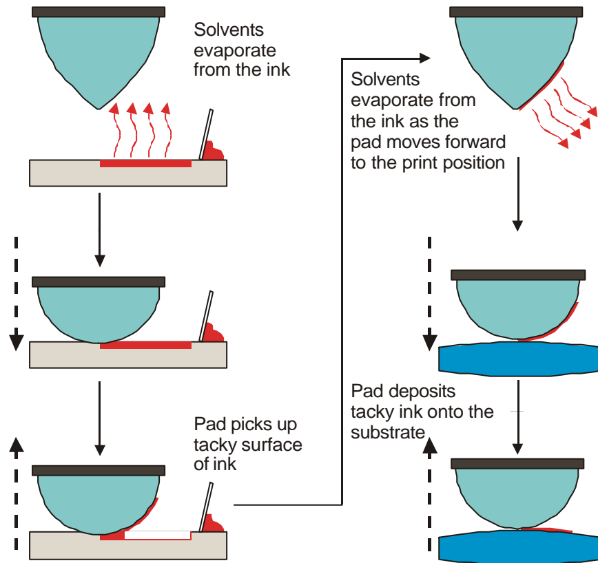
FIGURE 1.3 EVAPORATION OF THE SOLVENTS
