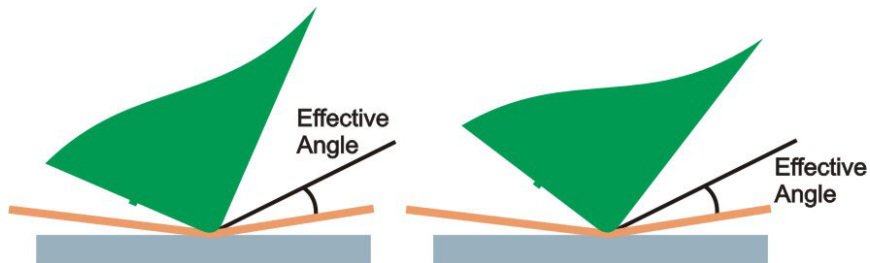
FIGURE 4. THE EFFECT OF MAJOR ANGLE CHANGE
