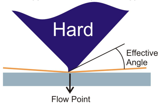
FIGURE 7. EFFECT OF HARDNESS
