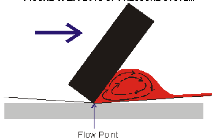
FIGURE 1. EFFECTS OF PRESSURE SYSTEM
